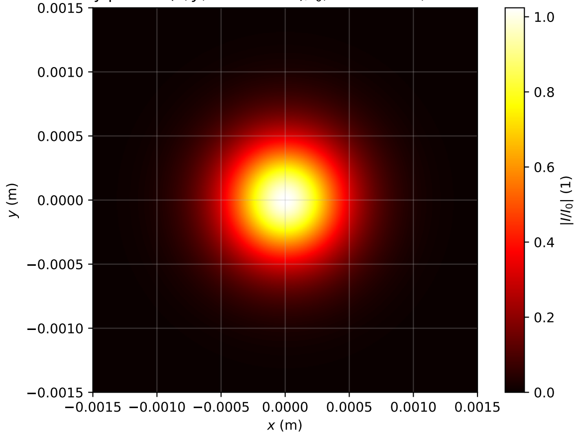
Intensity profile I(x, y, z = 1.194m)/I_0 , P_{in}=0.5P_{cr} , artificial time
